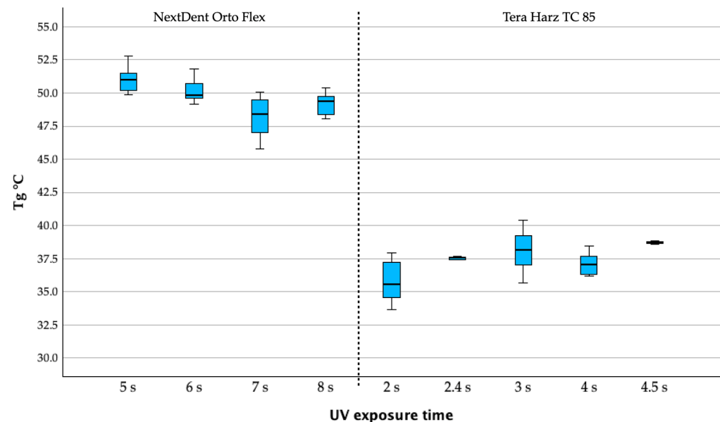
Figure 4. Glass transition temperature (°C).
